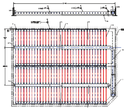
Biofilter Cell Arrangement
