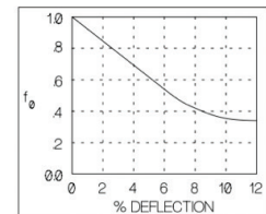
FIGURE 5 : OVALITY CORRECTION FACTOR
